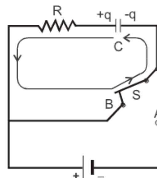
Fig. (iii) Discharging of a capacitor
