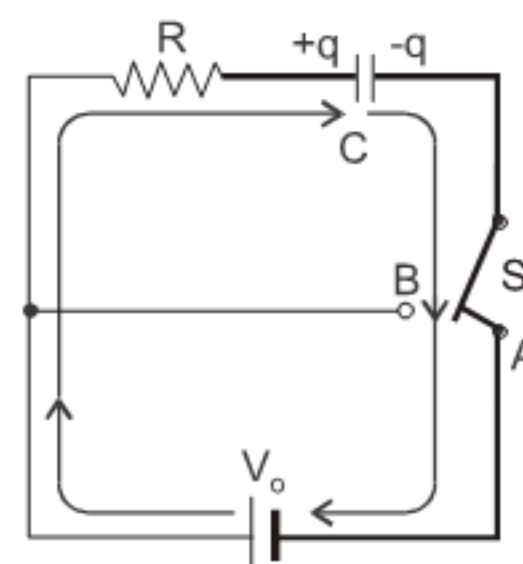
Fig. (i) Charging a capacitor
