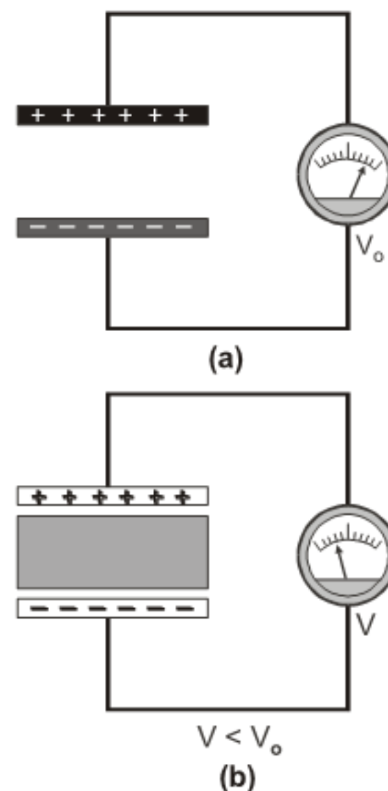
Fig. Effect of a dielectric on the capacitance of a capacitor.
