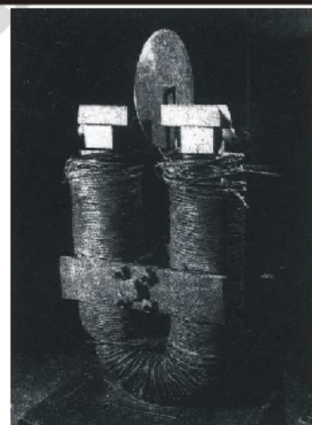
Faraday's homopolar generator with which he was able to produce a continuous induced current.
