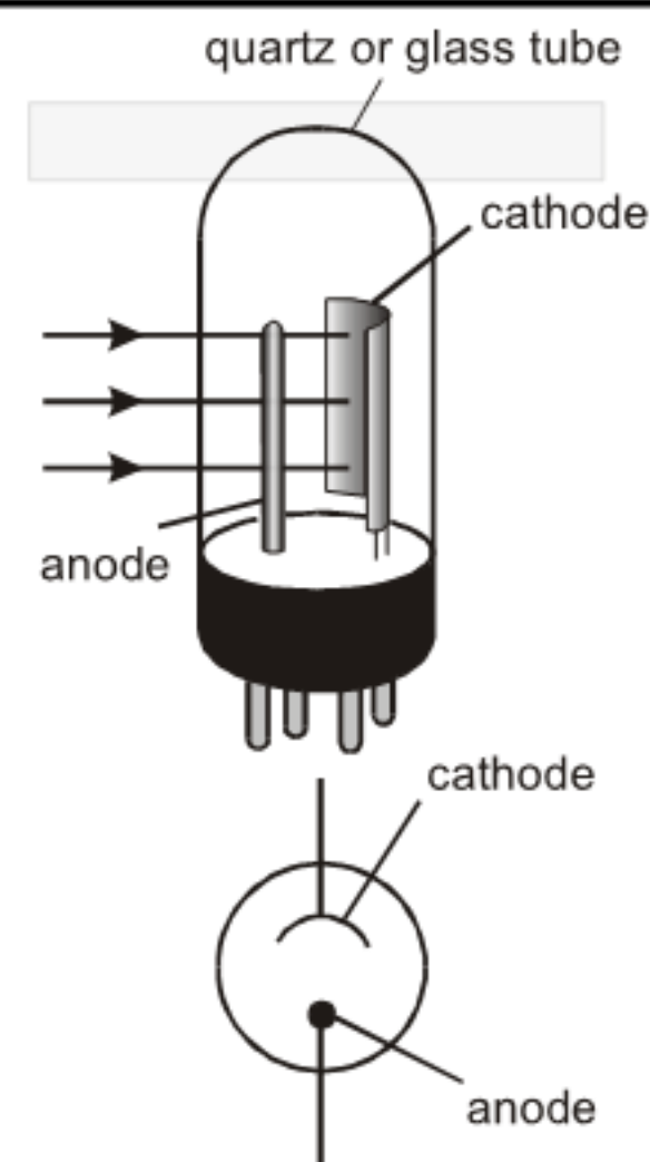
Fig. Simple photo-emissive cell
