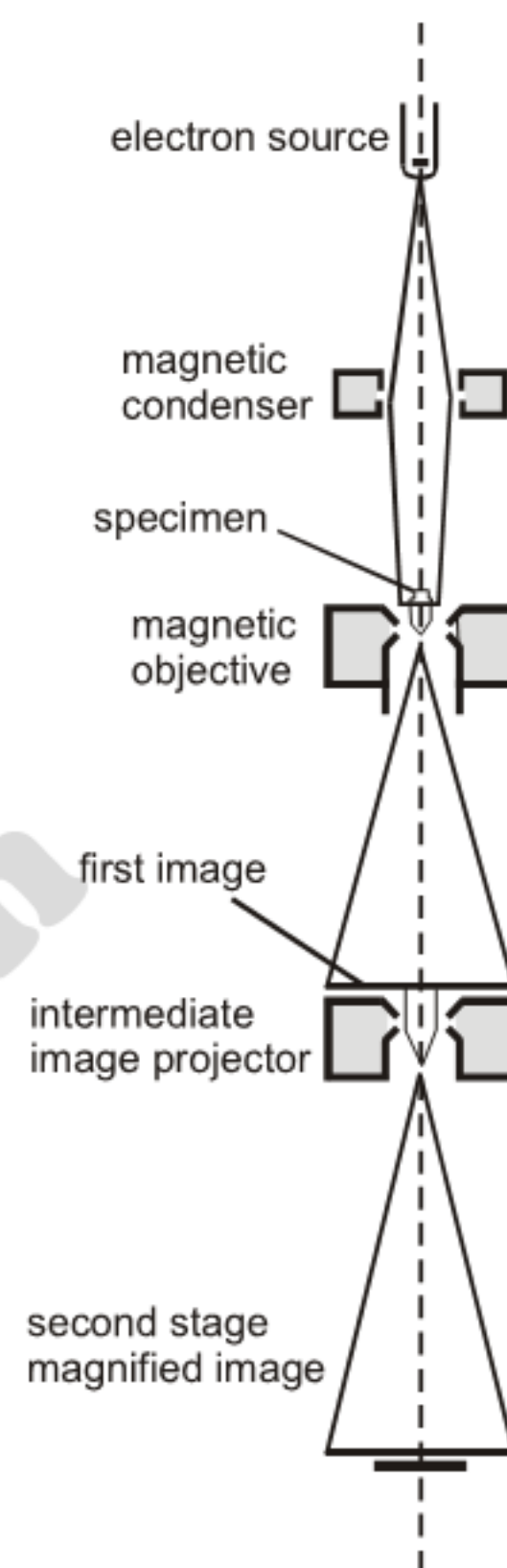
Fig. Electron microscope (Block diagram)
