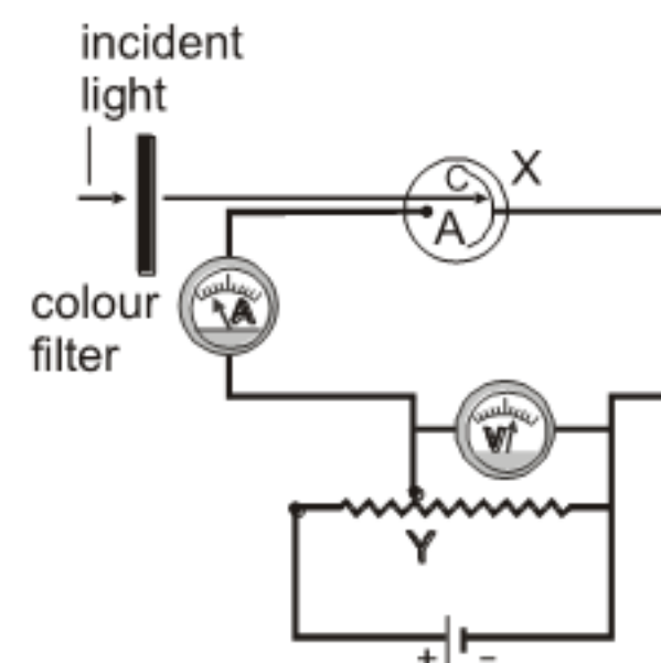
Fig. Experimental arrangement to observe photoelectric effect.
