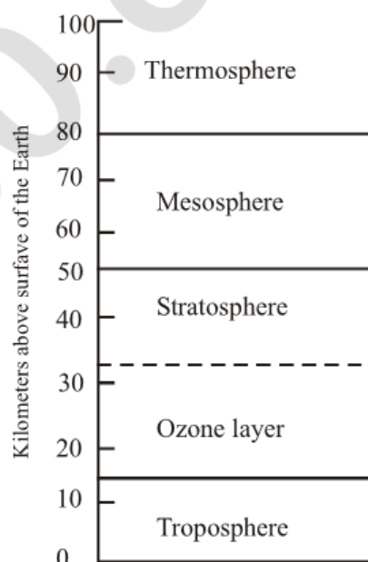
Division of the atmosphere and approximate location of the ozone layer
